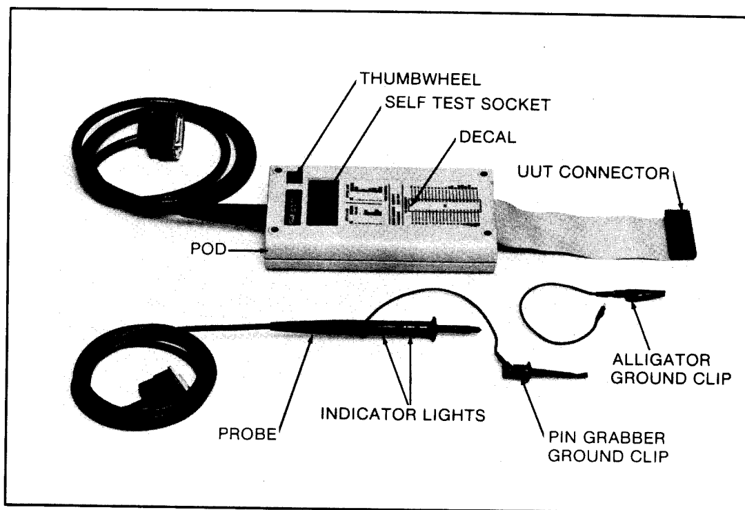
Figure 3B-4. Interface Pod and Probe
