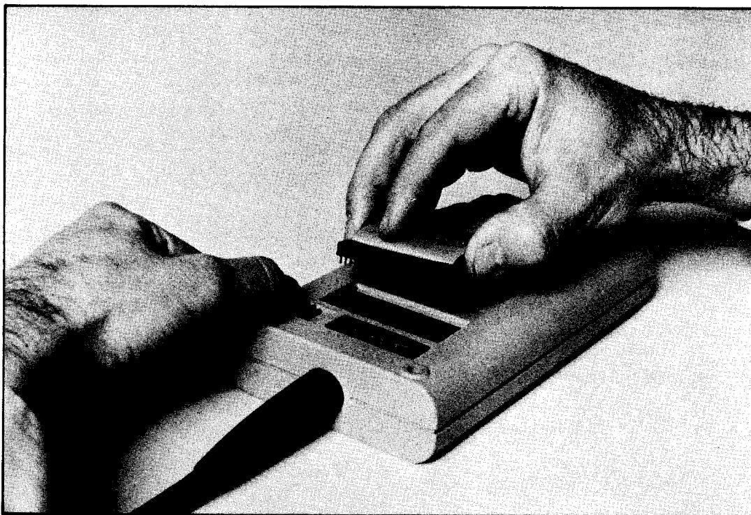
Figure 4A-2. Interface Pod Self Test Connection
