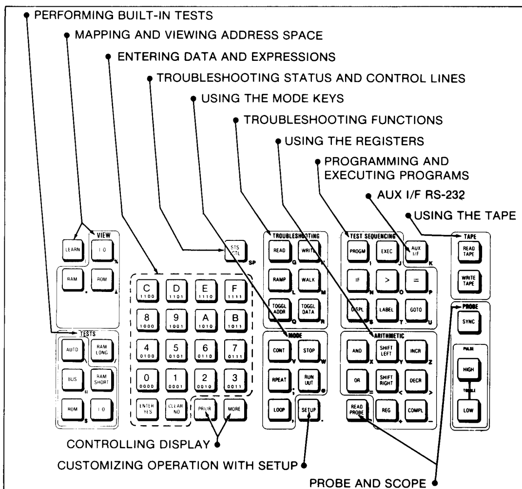
Figure 3C-1. 9010A Keyboard
