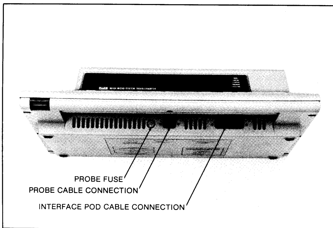
Figure 3B-3. Probe Fuse and Cable Connection
